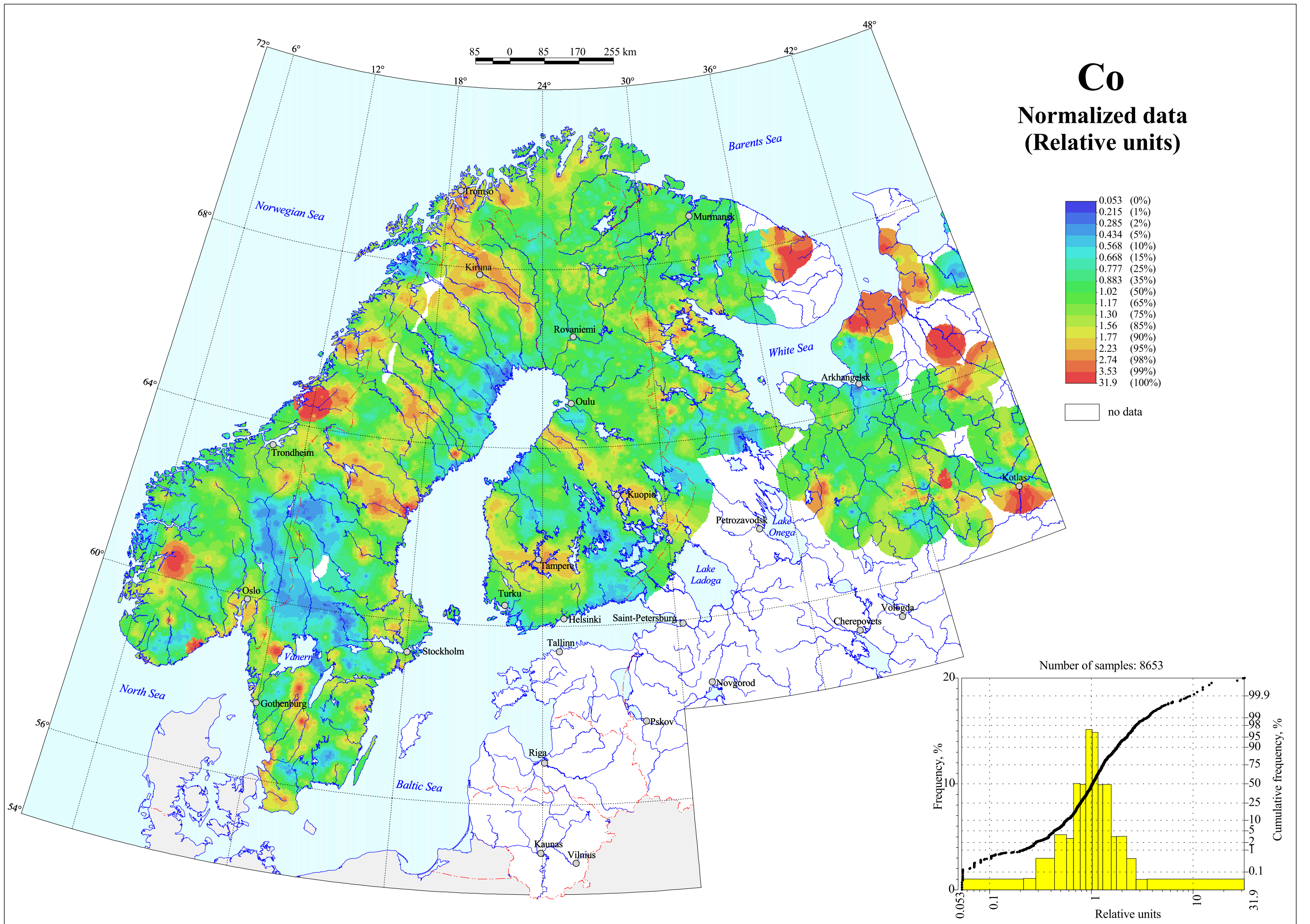
Cobalt in Till, Grain Size <0.06 mm
